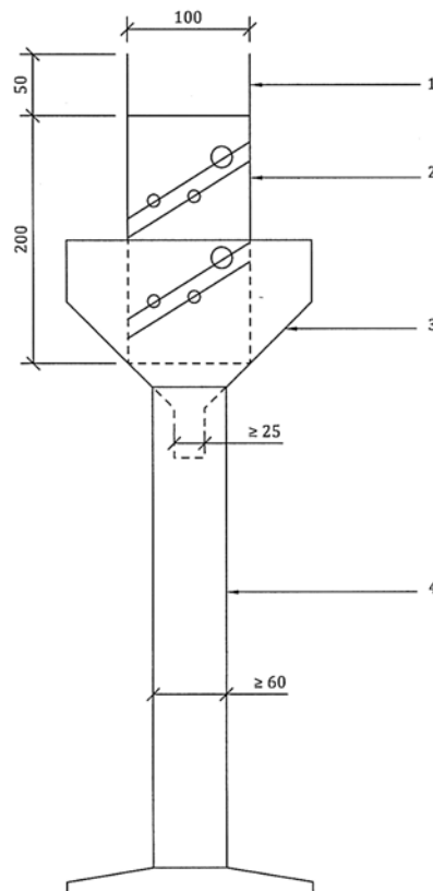
Fig 1: Test setup and Dimensions (all dimensions in mm)
