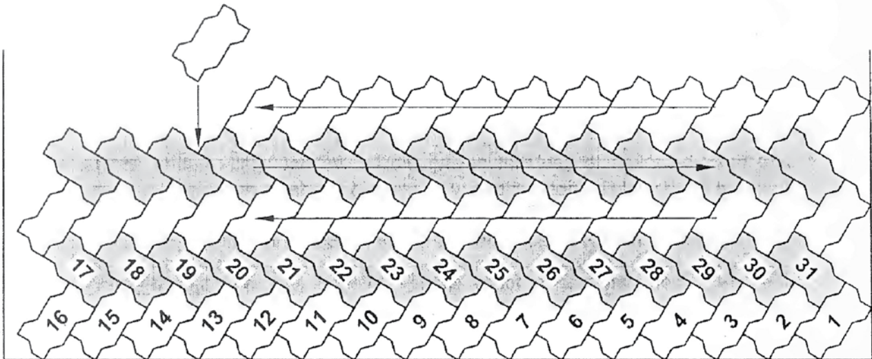
(A) AXIS OF UNITS NOT PARALLEL TO EDGE RESTRAINTS -ONLY ONE OPERATOR CAN WORK ON THE LAYING FACE
