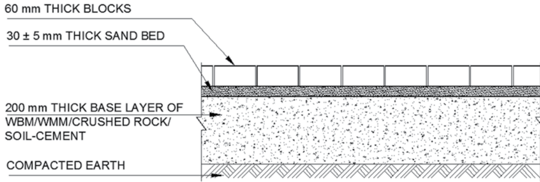
Fig. 5 A Typical Cross Section of Block Pavement used in Sidewalks/Footpaths/Car-Parks/Cycle Tracks
