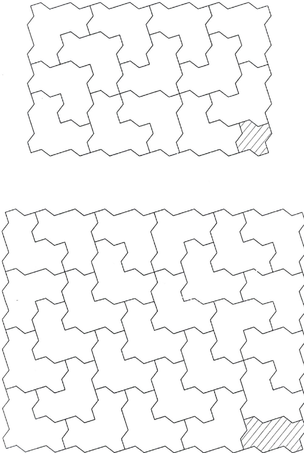
Fig. 16 Typical Block Cluster in Mechanised Laying
