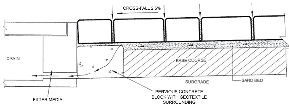
Fig. 9 Sub Surface Drainage in a Block Pavement
