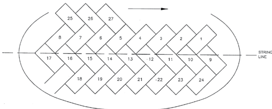
Fig. 13 Starting at Irregular Shaped Edge Restraint
