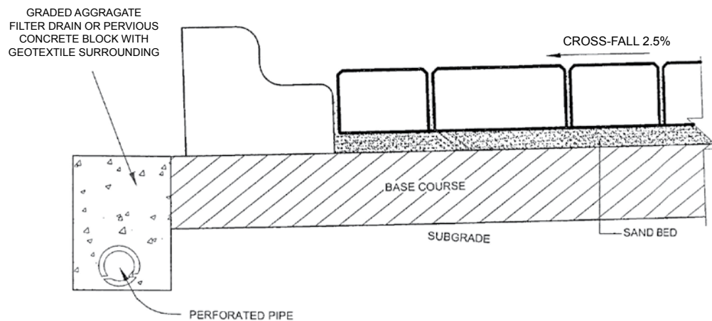
Fig. 10 Sub Surface Drainage in a Block Pavement
