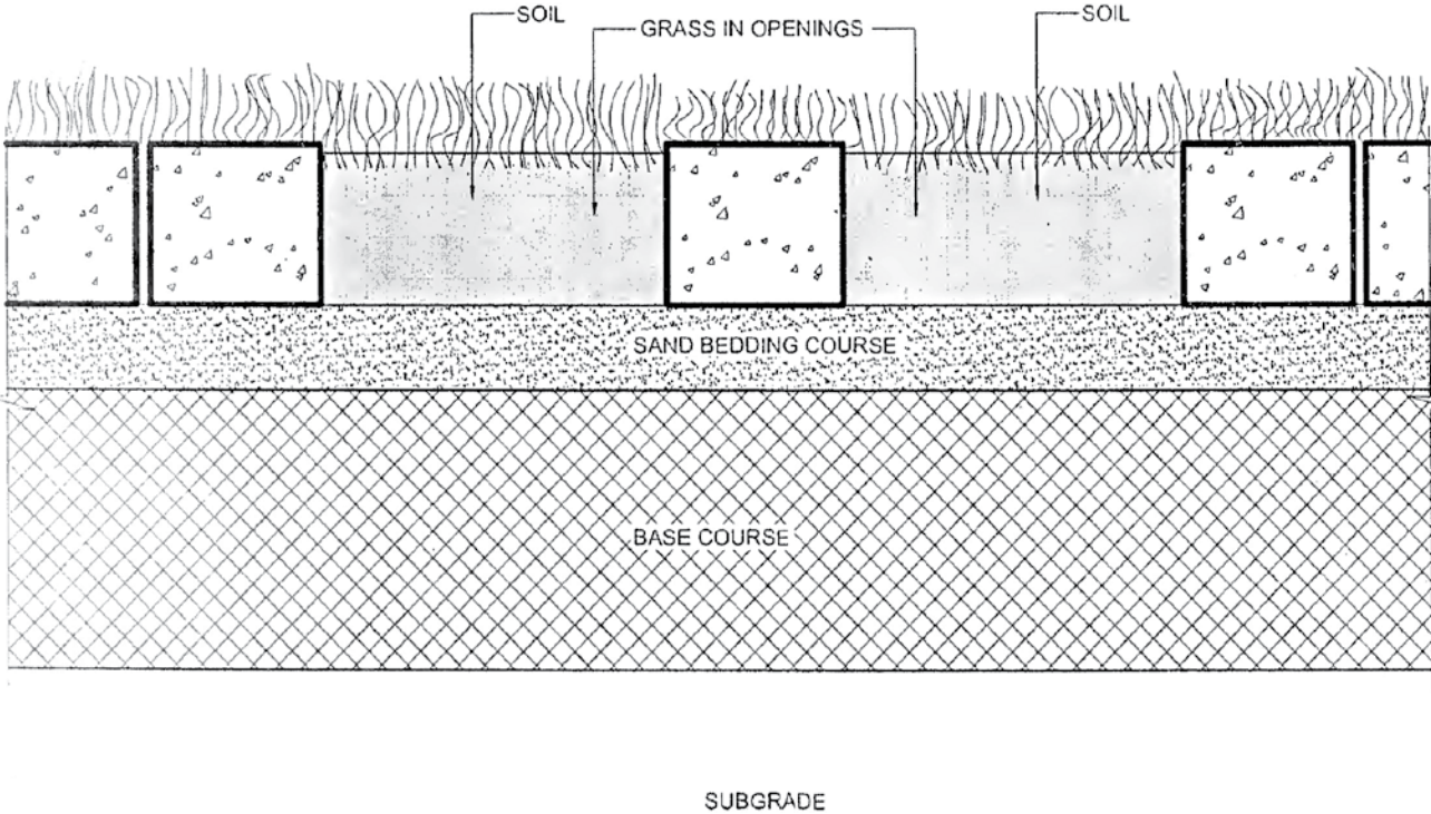
Fig. 4 Grass Blocks and Construction Technique
