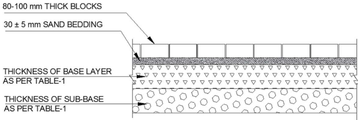
Fig. 6 A Typical Cross Section of Block Pavement for Medium and Heavily Trafficked Roads except National-Highways, Expressways, State Highways and MDR
