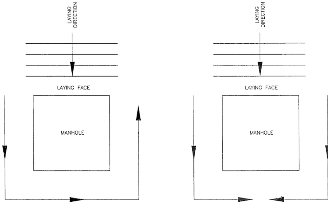
Fig. 20. Laying Block Paving Around a Manhole
