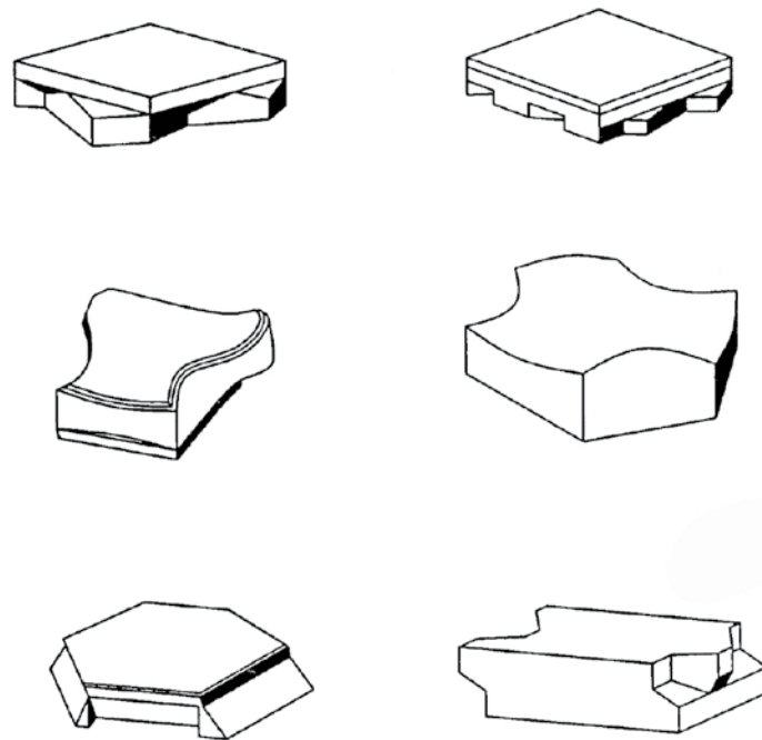
(ii) SOME TYPICAL SHAPES OF VERTICALLY INTERLOCKING BLOCKS
