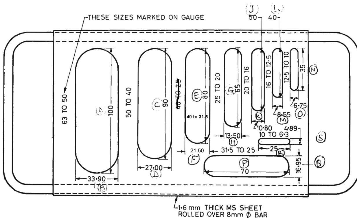
FIG. 2 THICKNESS GAUGE
