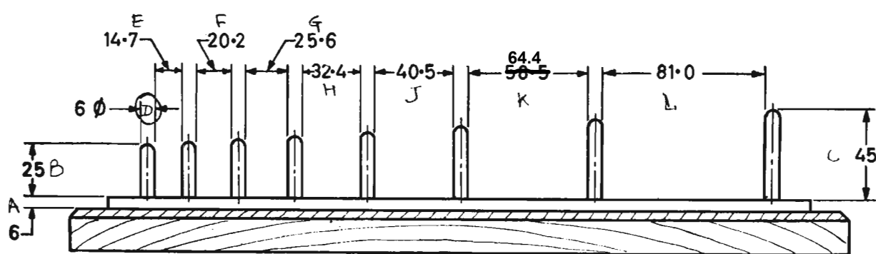
FIG. 3 LENGTH GAUGE
