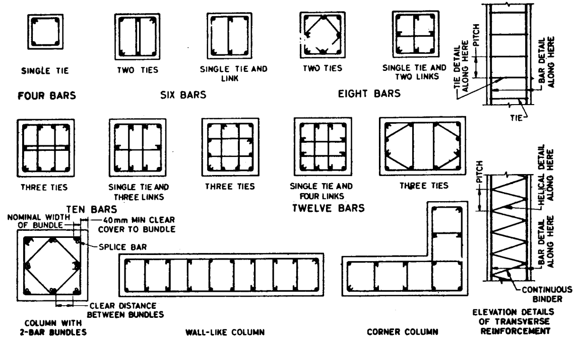
FIG. 7 TYPICAL ARRANGEMENT OF LATERAL TIES AND LINKS IN COLUMNS
