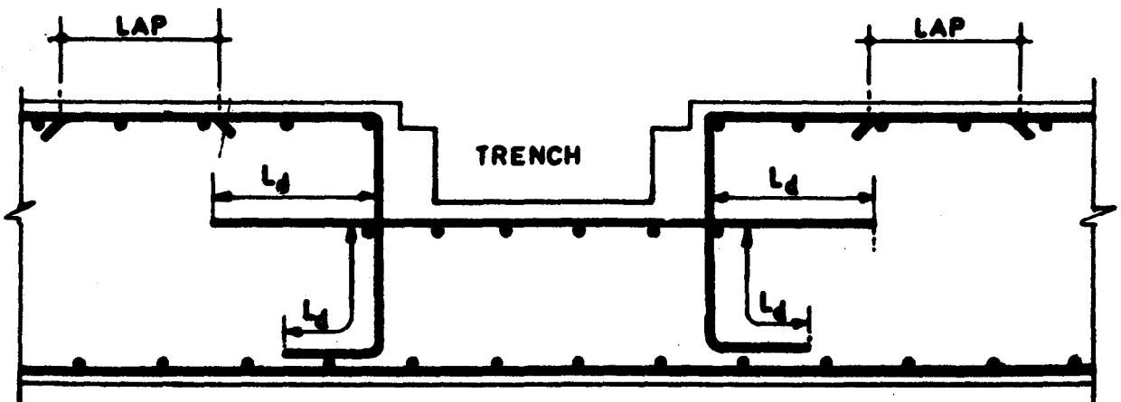
FIG. 6.6 TYPICAL DETAILS AROUND A TRENCH IN RAFT FOUNDATION
