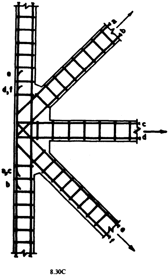
FIG. 8.30 TIE END CONNECTIONS FOR LIGHT LOADING
