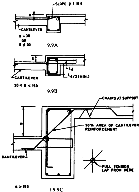
FIG. 9.8 CANTILEVER SLABS AT THE BOTTOM OF BEAMS
