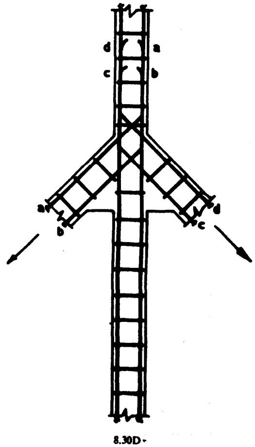
FIG. 8.30 TIE END CONNECTIONS FOR LIGHT LOADING
