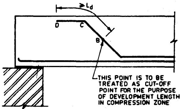
4.2B IN COMPRESSION ZONE
