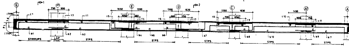
BEAM ALONG GRID 1 & 13
