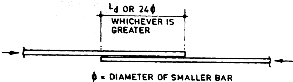
IN COMPRESSION
