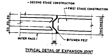
TYPICAL DETAIL OF EXPANSION JOINT
