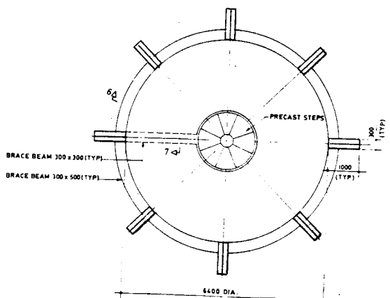
PLAN OF STAGING SHOWING COLUMNS & BRACINGS
