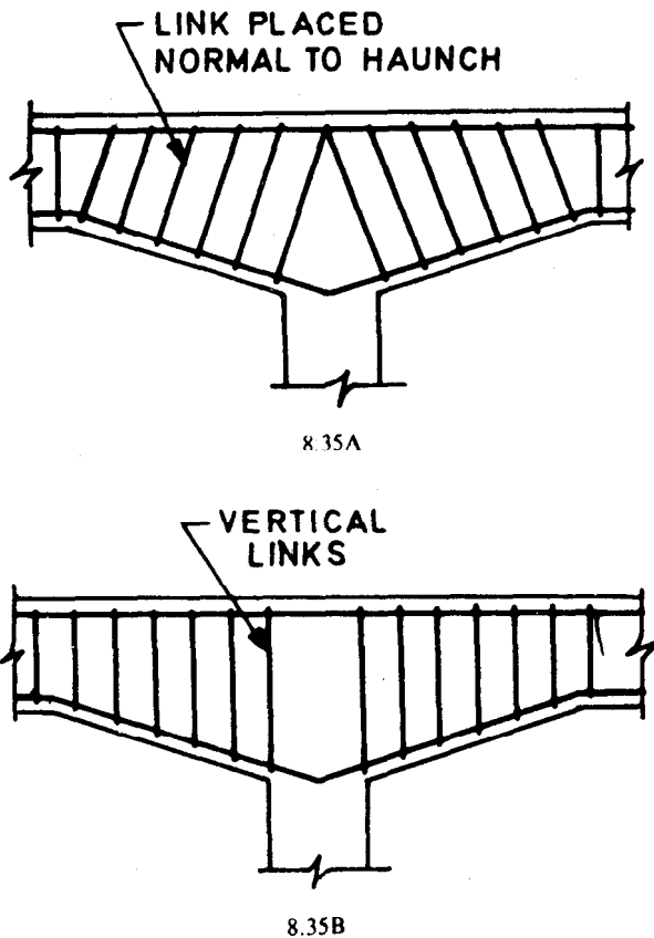
FIG. 8.35 LINKS OR TIES IN HAUNCHS
