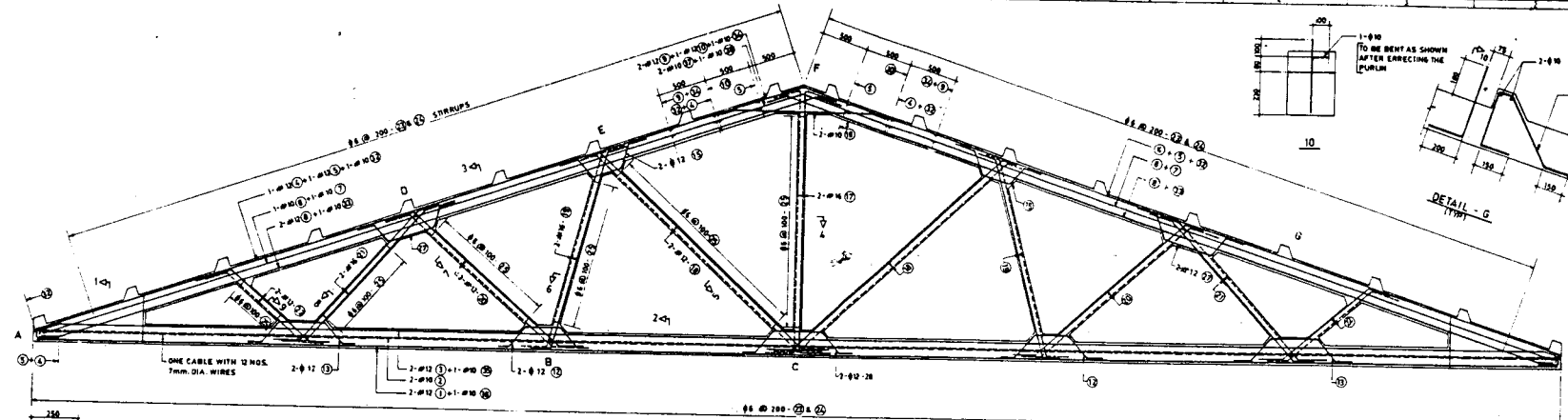
ELEVATION OF PRECAST TRUSS
