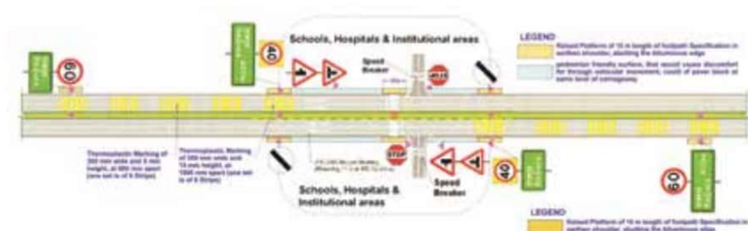
Fig. 7.21 Schematic Diagram for Highway Corridors
