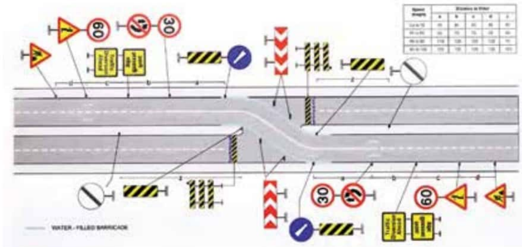
Fig. 7.16 Two Lane to Four Lane (Shifting of Traffic from One Carriageway to the other)
