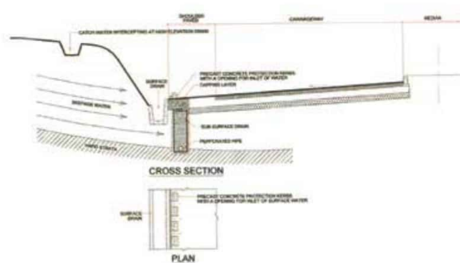
Fig. 10.8 Surface and Subsurface Drainage in Hill Section
