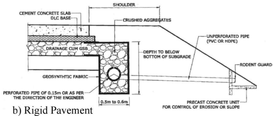
Fig. 10.6 Drainage Layer Terminated at Pavement Edge
